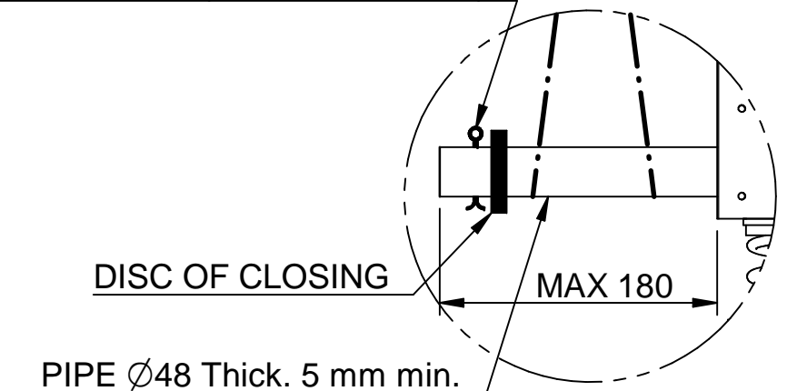
DETAIL B
